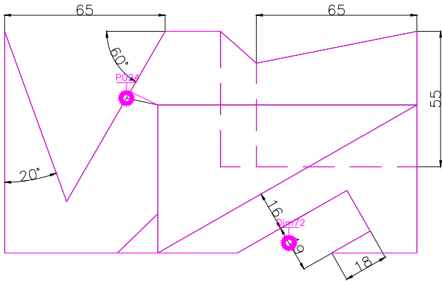
TOP SCALE 1/2
