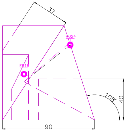
RIGHT SCALE 1/2
