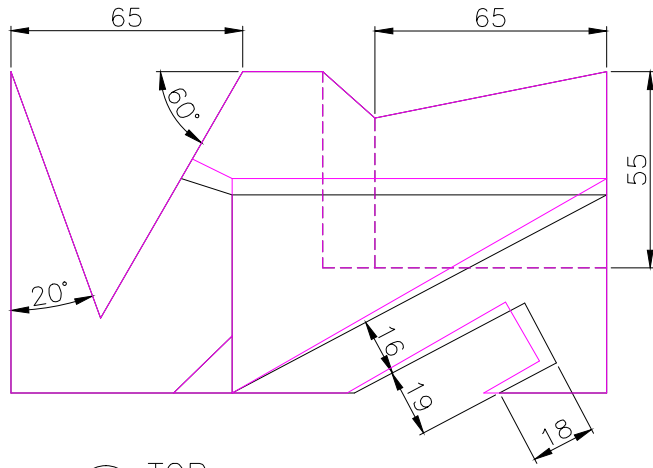
TOP SCALE 1/2
