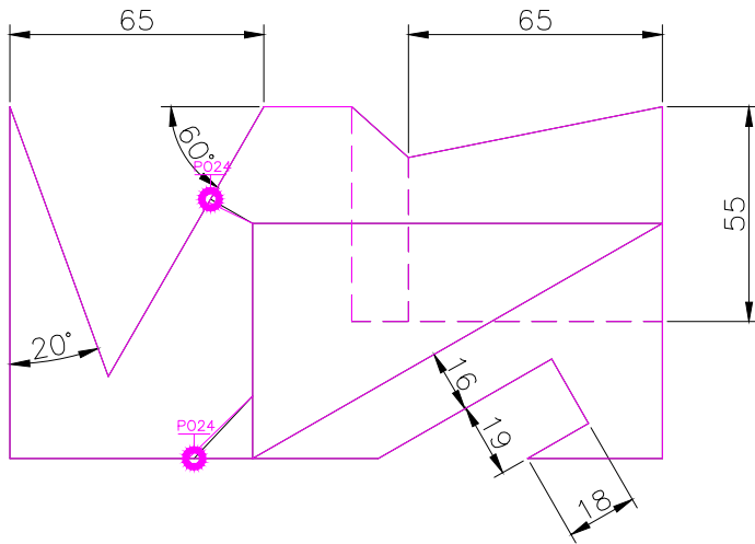
TOP SCALE 1/2
