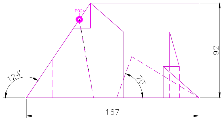
FRONT SCALE 1/2
