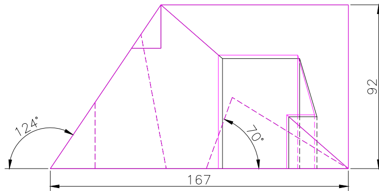
FRONT SCALE 1/2
