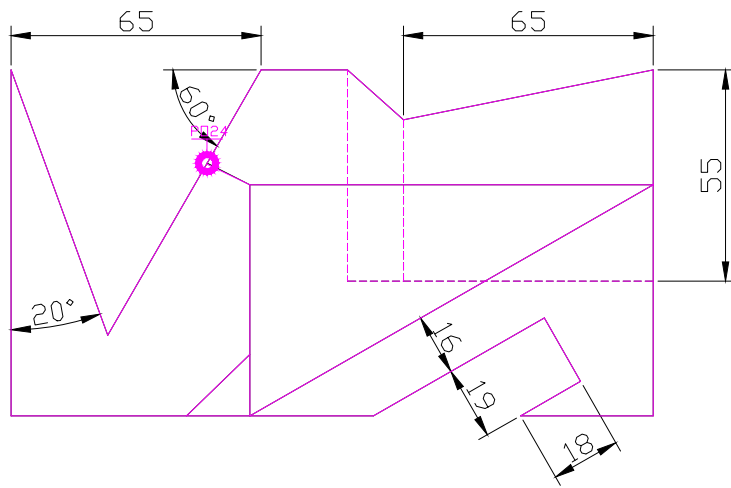
TOP SCALE 1/2
