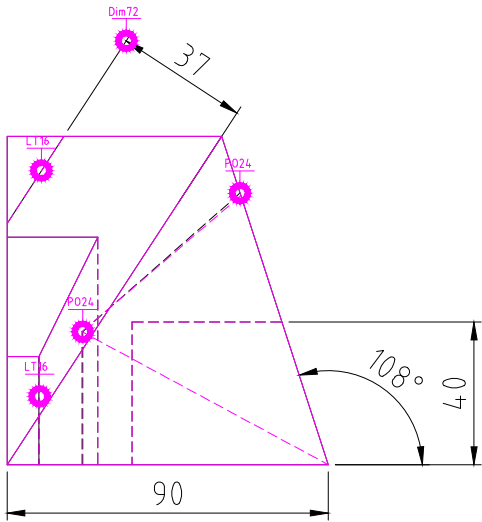
RIGHT SCALE 1/2
