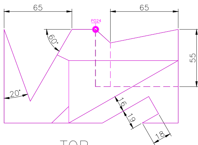
TOP SCALE 1/2
