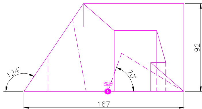
FRONT SCALE 1/2
