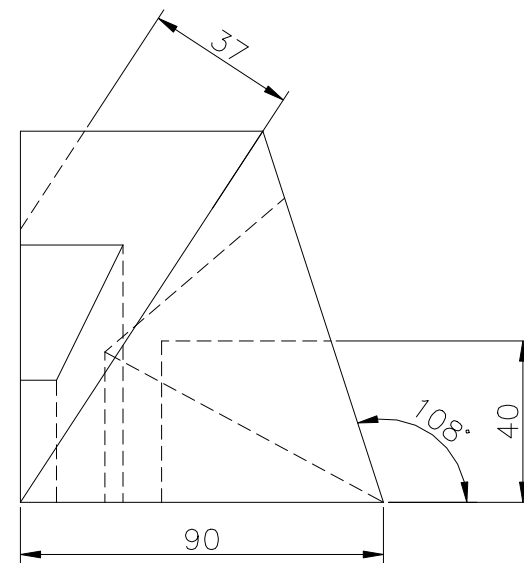
RIGHT SCALE 1/2
