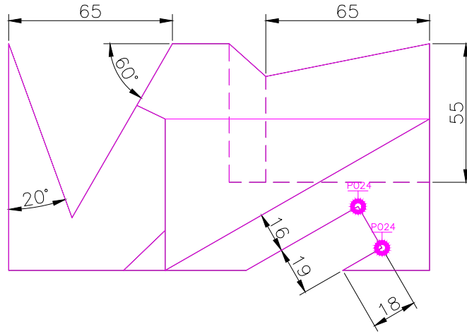
TOP SCALE 1/2
