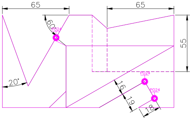
TOP SCALE 1/2
