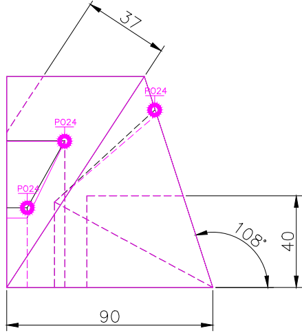
RIGHT SCALE 1/2
