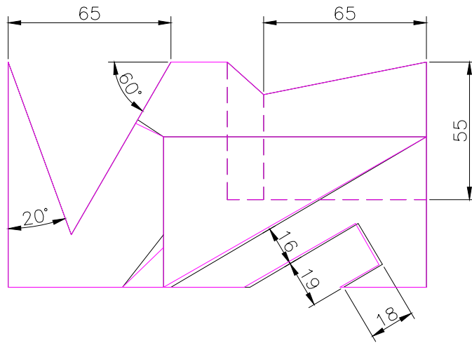
TOP SCALE 1/2
