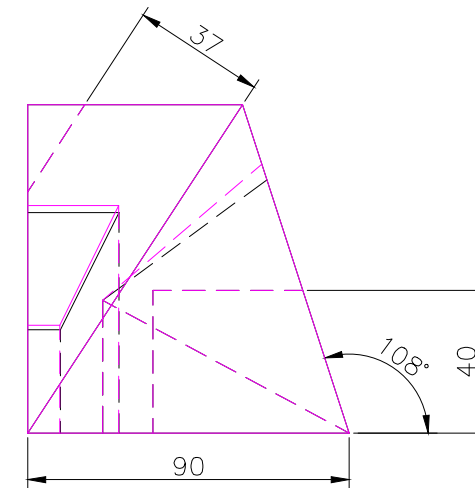
RIGHT SCALE 1/2
