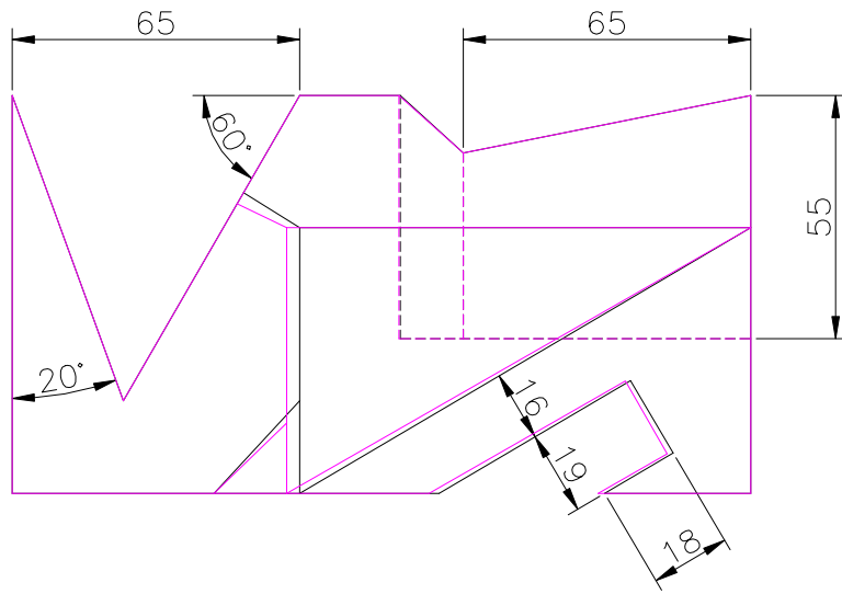
TOP SCALE 1/2
