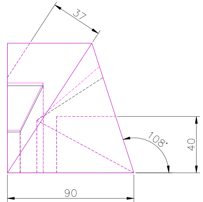
RIGHT SCALE 1/2
