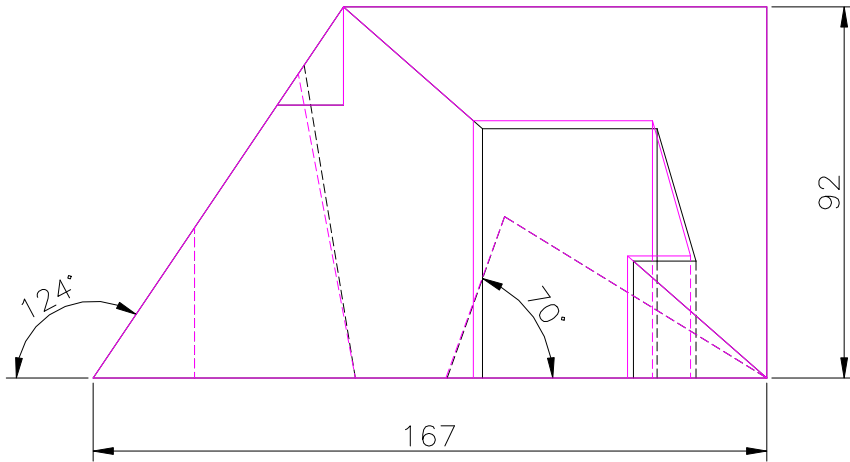
FRONT SCALE 1/2
