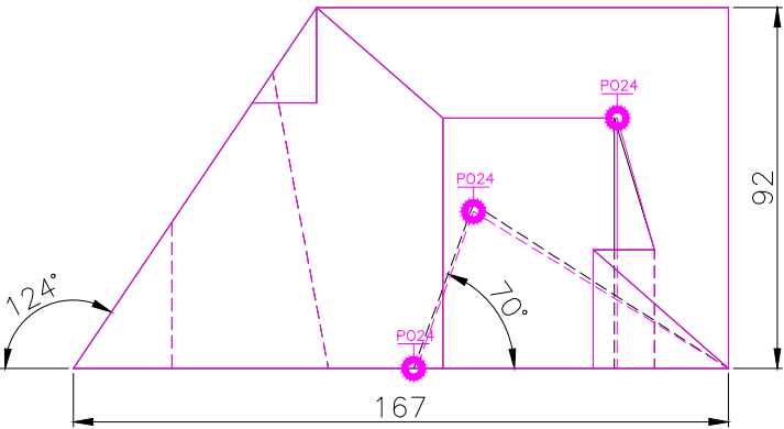
FRONT SACLE
