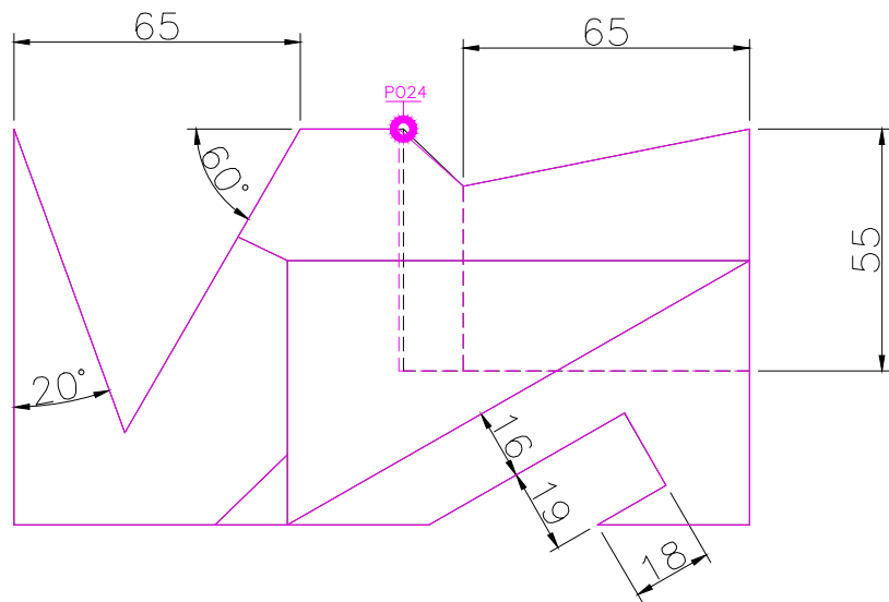
TOP SCALE 1/2
