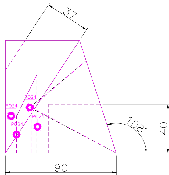
RIGHT SCALE 1/2
