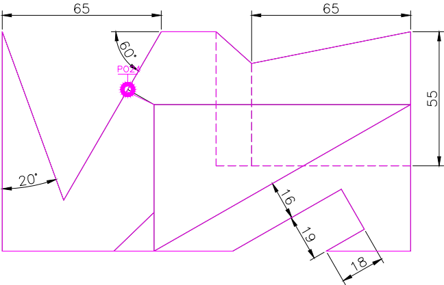
TOP SCALE 1/2
