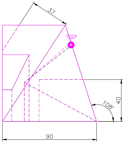
RIGHT SCALE 1/2
