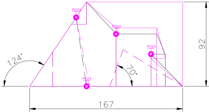
FRONT SCALE 1/2
