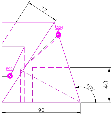
RIGHT SCALE 1/2
