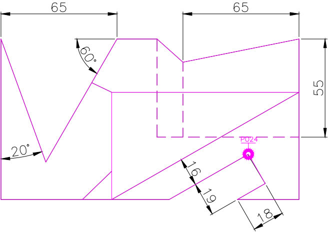
TOP SCALE 1/2
