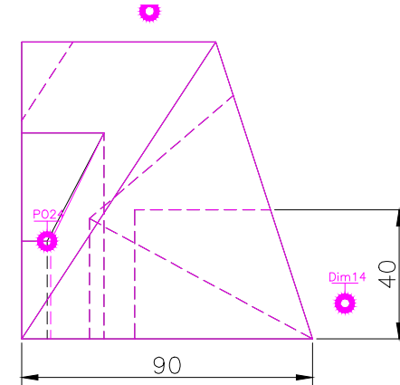
RIGHT SCALE 1/2
