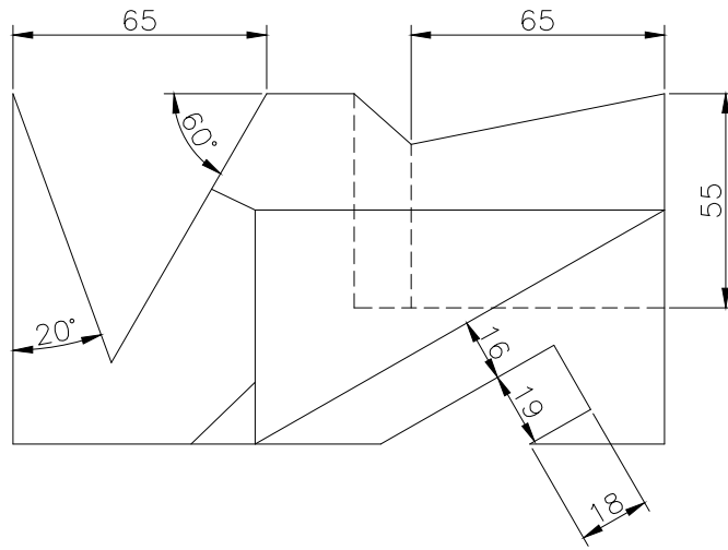
TOP SCALE 1/2
