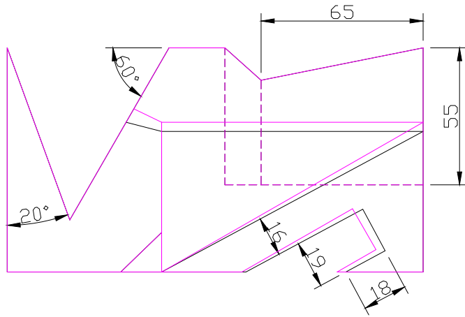
TOP SCALE 1/2
