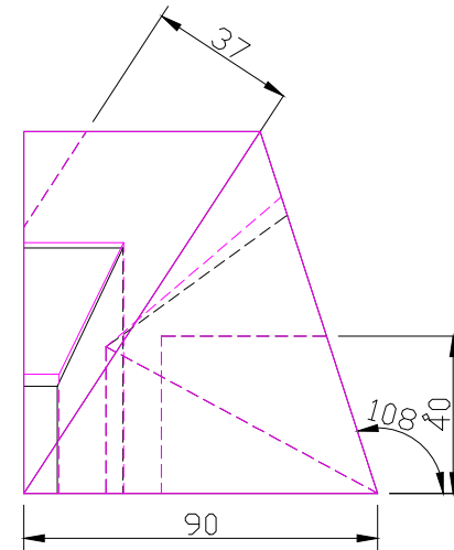
RIGHT SCALE 1/2
