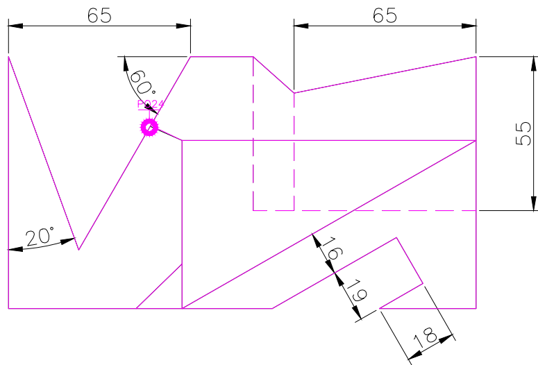
TOP SCALE 1/2
