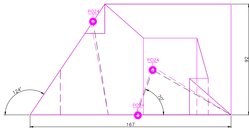
FRONT SCALE 1/2
