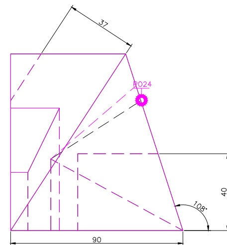
RIGHT SCALE 1/2
