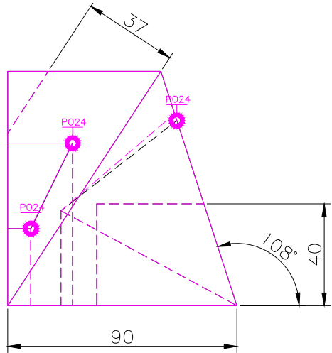
RIGHT SCALE 1/2
