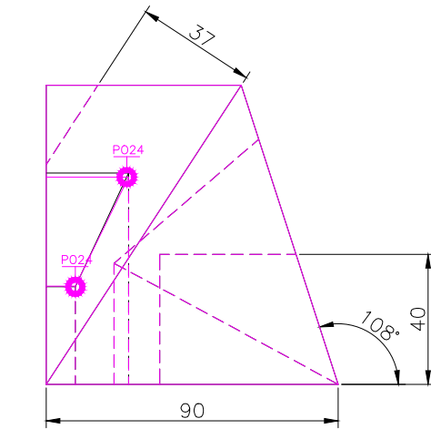
RIGHT SCALE 1/2
