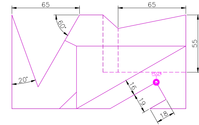
TOP SCALE 1/2
