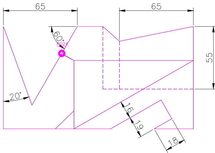
TOP SCALE 1/2
