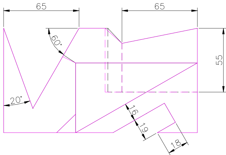
TOP SCALE 1/2
