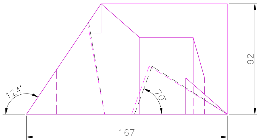
FRONT SCALE 1/2
