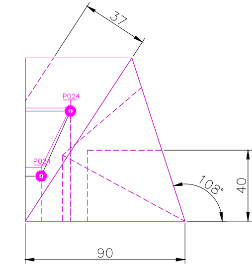
RIGHT SCALE 1/2
