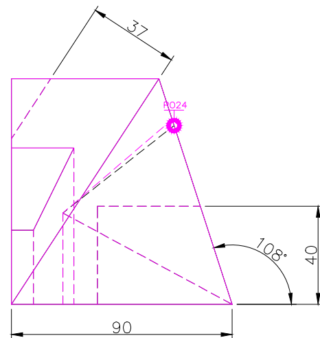
RIGHT SCALE 1/2
