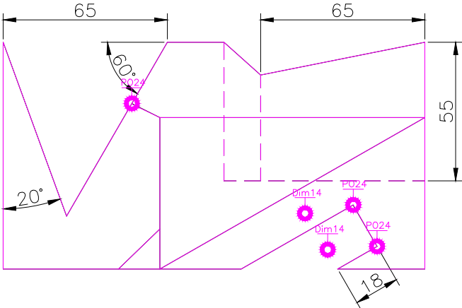
FRONT SCALE 1/2
