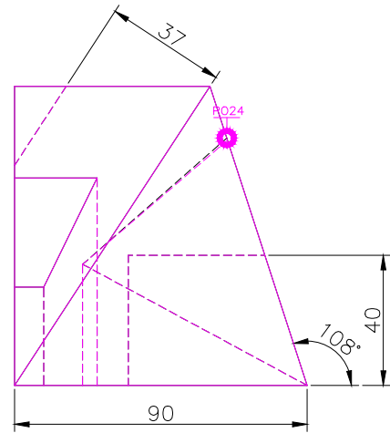
RIGHT SCALE 1/2
