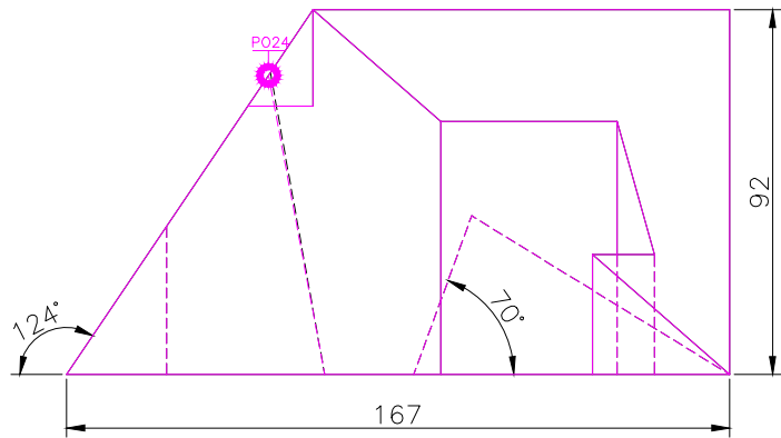
FRONT SCALE 1/2
