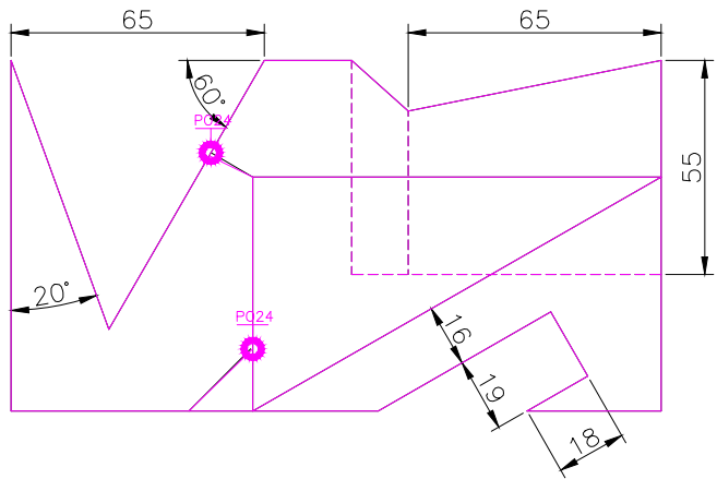
TOP SCALE 1/2
