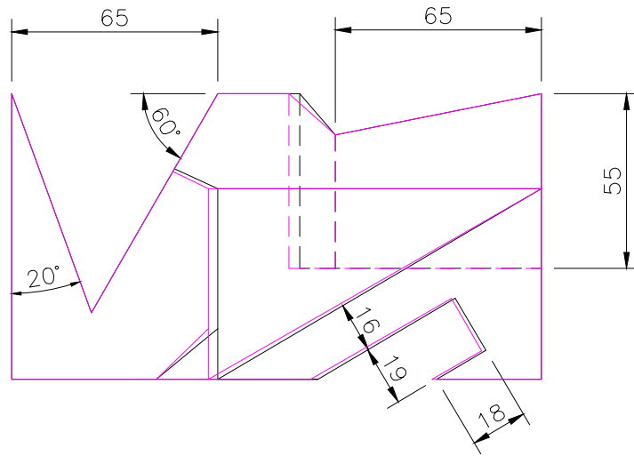
TOP SCALE 1/2
