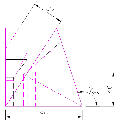
RIGHT SCALE 1/2
