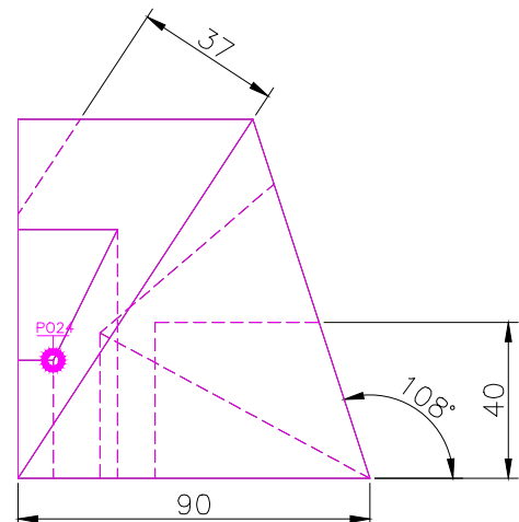
RIGHT SCALE 1/2
