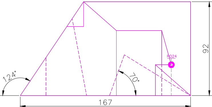
FRONT SCALE 1/2
