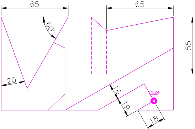
TOP SCALE 1/2
