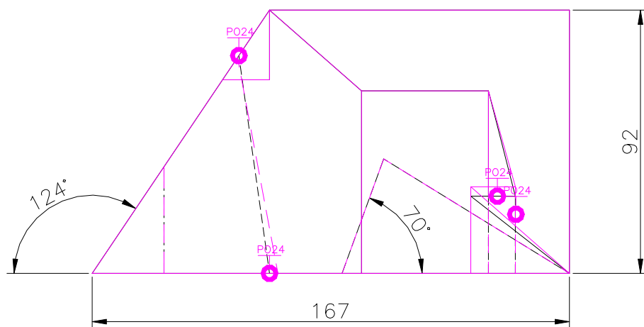
FRONT SCALE 1/2
