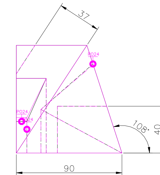
RIGHT SCALE 1/2
