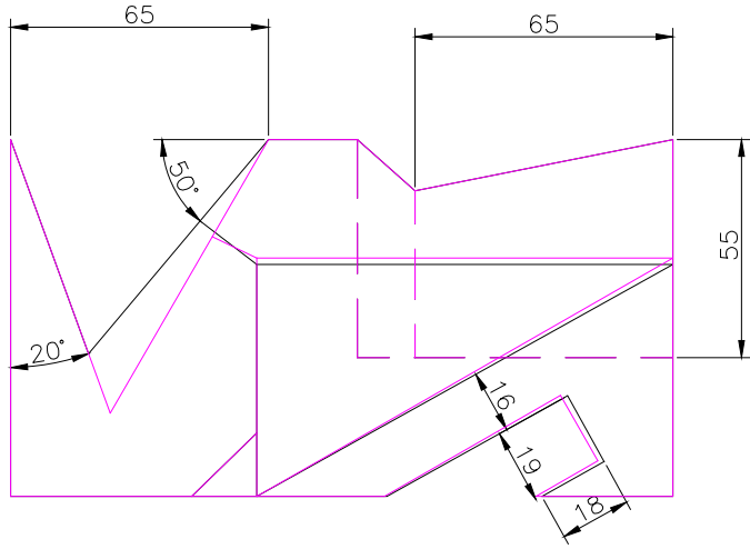
TOP SCALE 1/2
