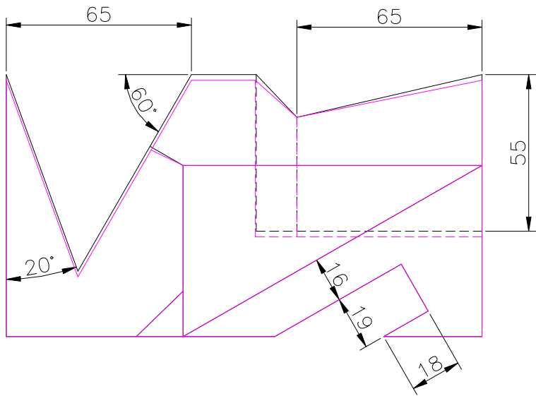
TOP SCALE 1/2
