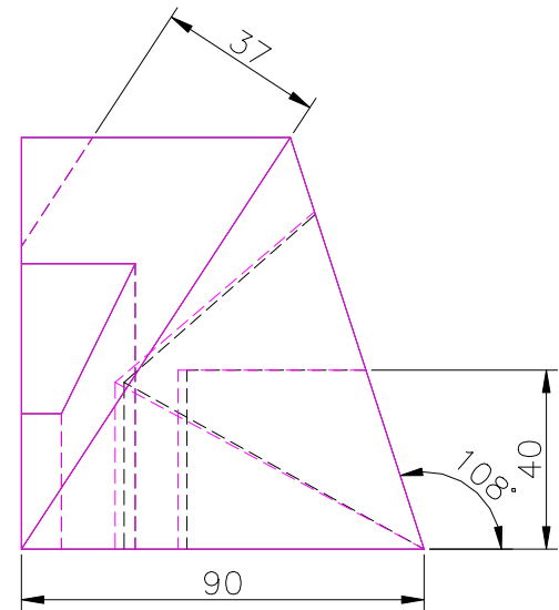
RIGHT SCALE 1/2
