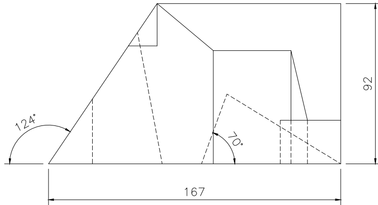
FRONT SCALE 1/2
