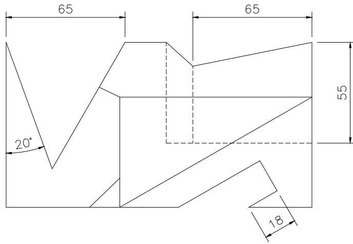
TOP SCALE 1/2
