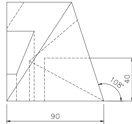
RIGHT SCALE 1/2
