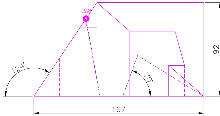
FRONT SCALE 1/2
