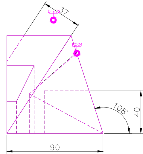
RIGHT SCALE 1/2
