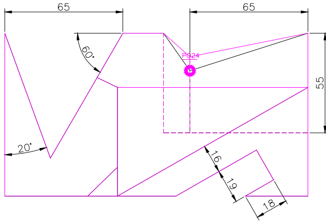
TOP SCALE 1/2
