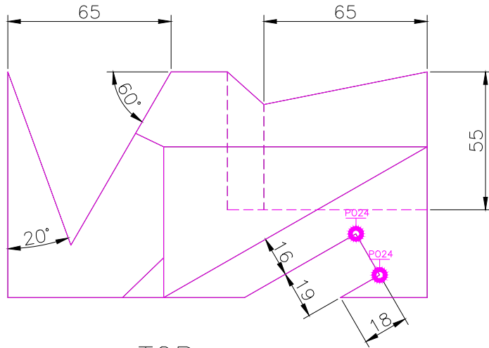
TOP SCALE 1/2
