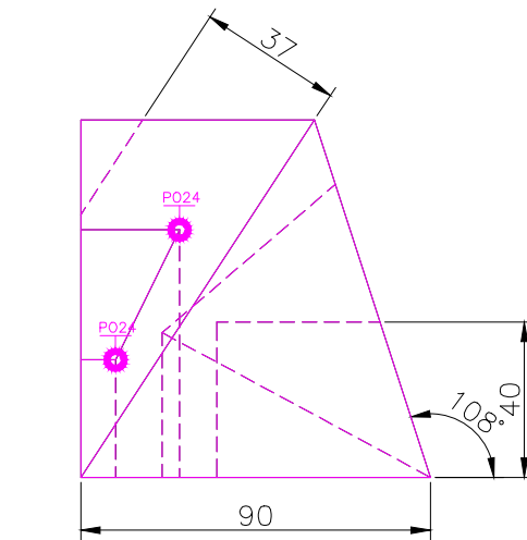
RIGHT SCALE 1/2
