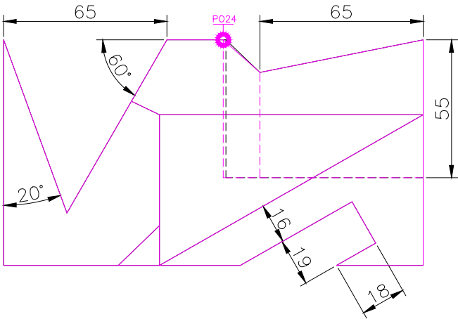
TOP SCALE 1/2
