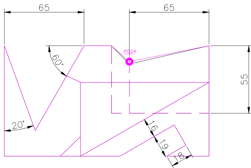
TOP SCALE 1/2
