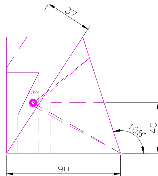
RIGHT SCALE 1/2
