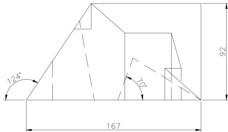
FRONT SCALE 1/2
