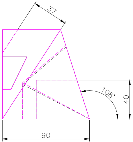
RIGHT SCALE 1/2
