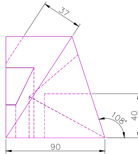
RIGHT SCALE 1/2
