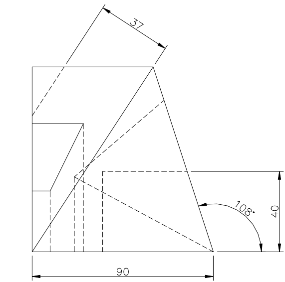
RIGHT SCALE 1/2
