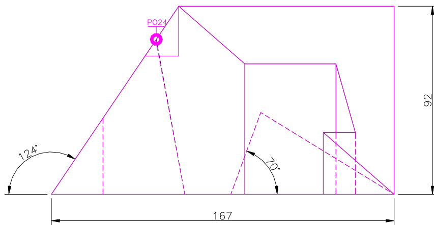
FRONT SCALE 1/2
