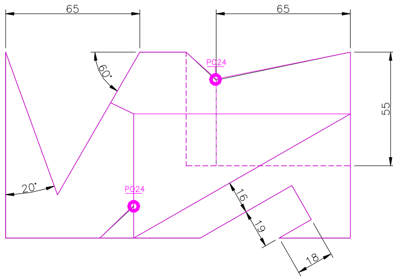
TOP SCALE 1/2
