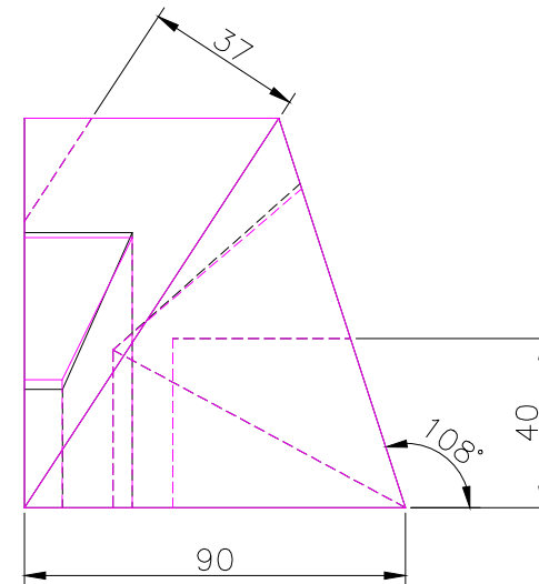
RIGHT SCALE 1/2
