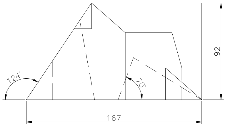
FRONT SCALE 1/2
