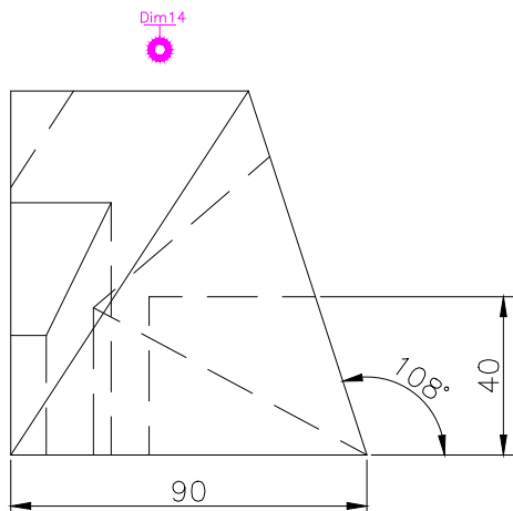
RIGHT SCALE 1/2
