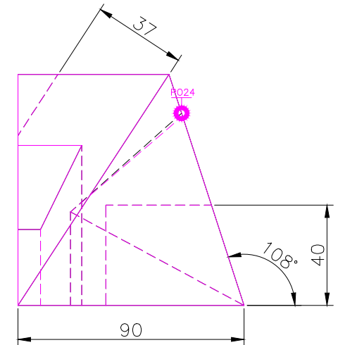
RIGHT SCALE 1/2
