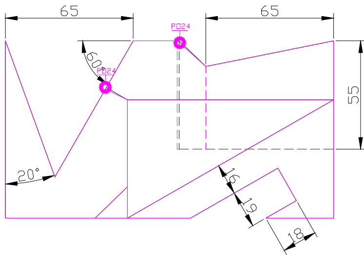
TOP SCALE 1/2
