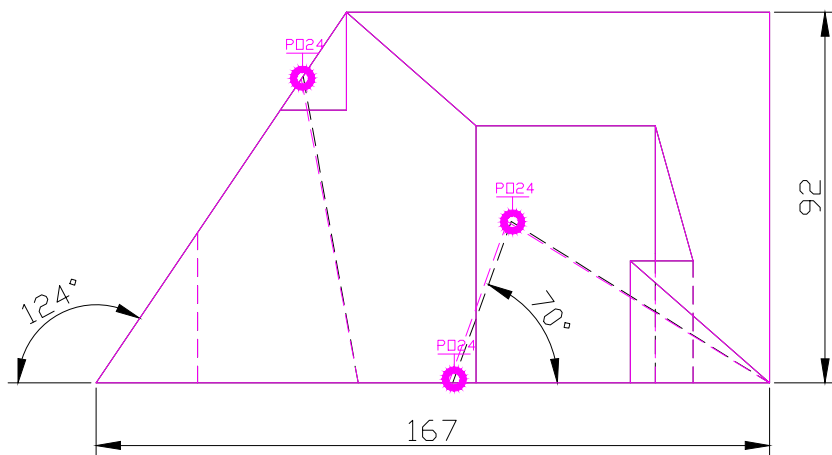
FRONT SCALE 1/2
