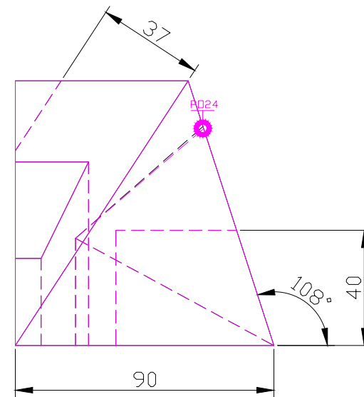
RIGHT SCALE 1/2
