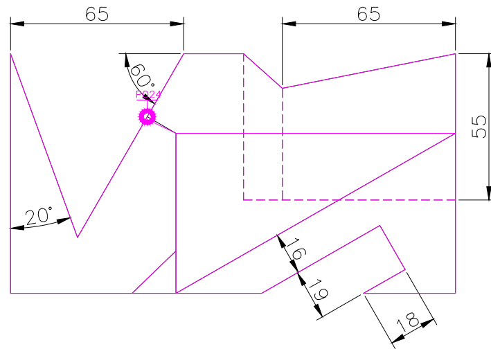
TOP SCALE 1/2
