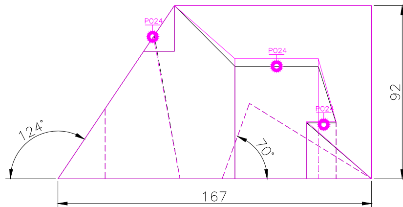
FRONT SCALE 1/2
