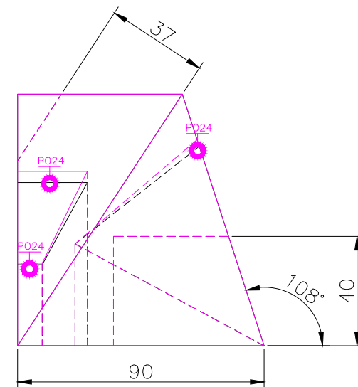
RIGHT SCALE 1/2
