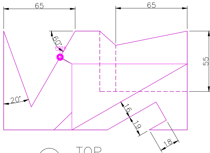
TOP SCALE 1/2
