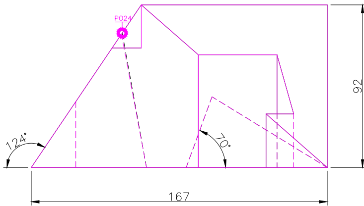
FRONT SCALE 1/2
